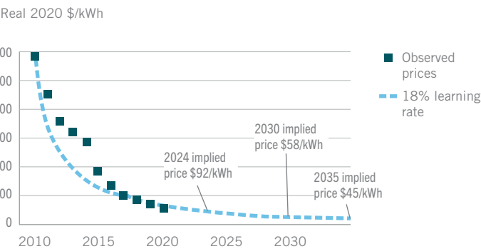
FIGURE 30: Lithium-ion battery pack price
