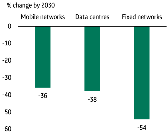
Figure 25: ...which should be reduced to align with the Paris Agreement target
